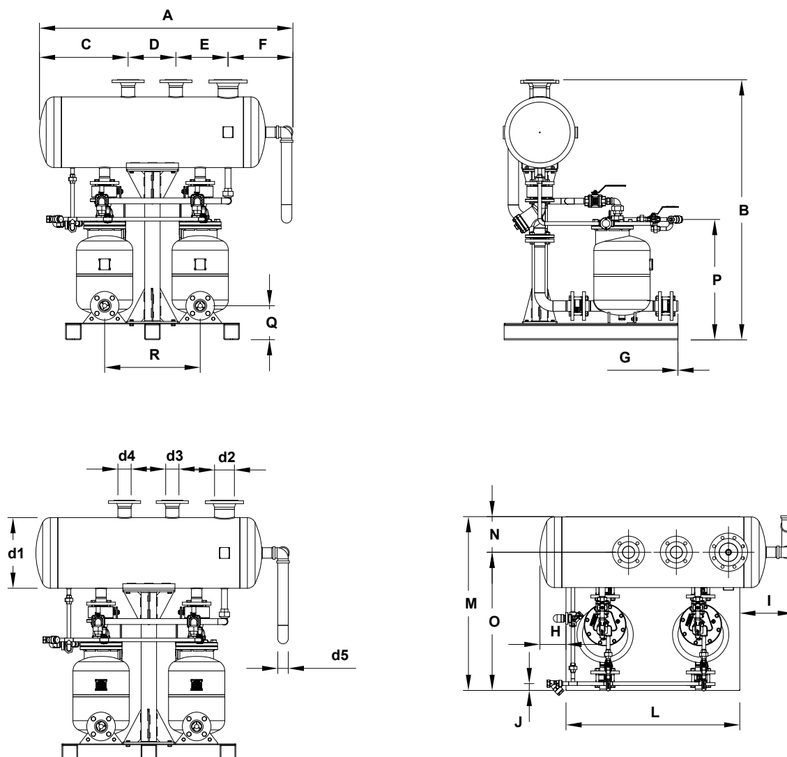
DIMENSIONS (mm)
