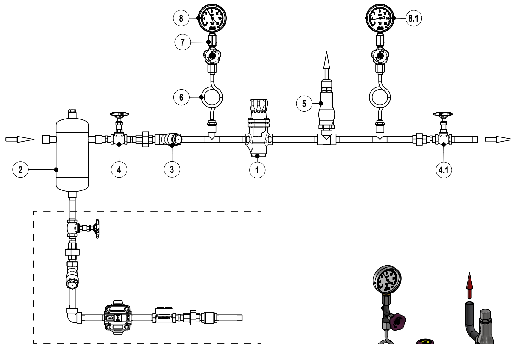
Steam trap installation
